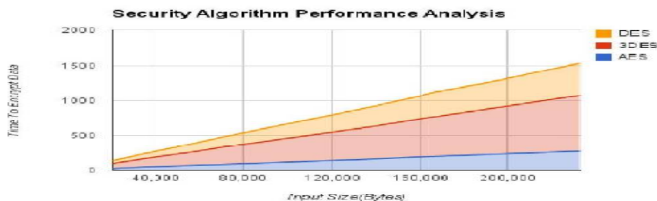
Fig.2.Performance Analysis for Security Algorithm
