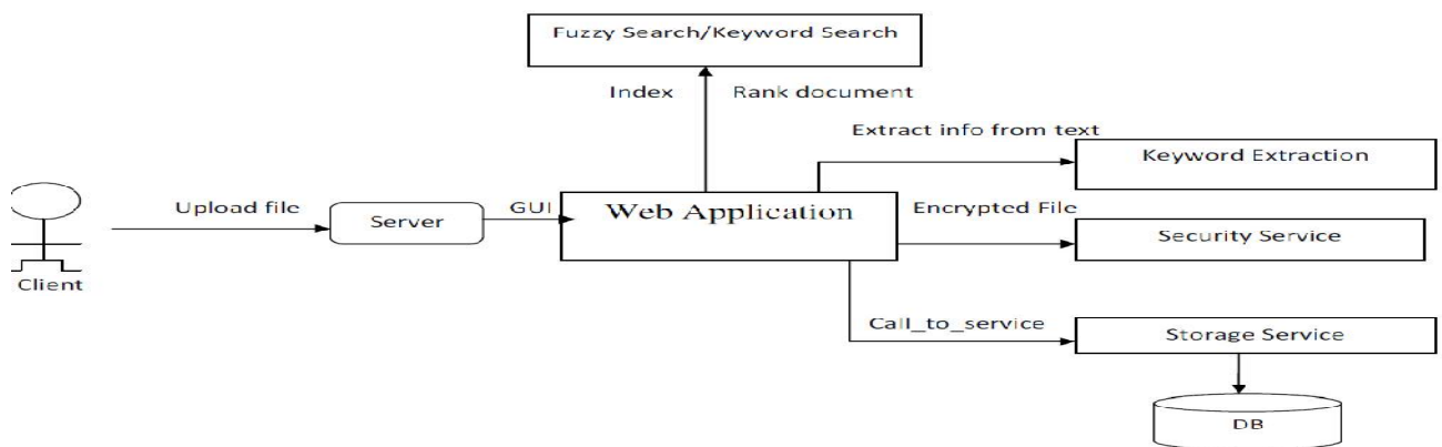
Fig.1. Architecture of Proposed System
