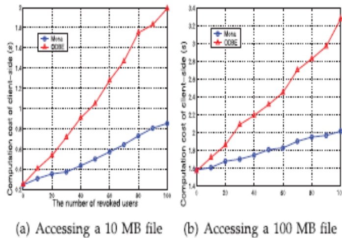
Fig. 3. Comparison on client computation cost for file access between this scheme and ODBE.
