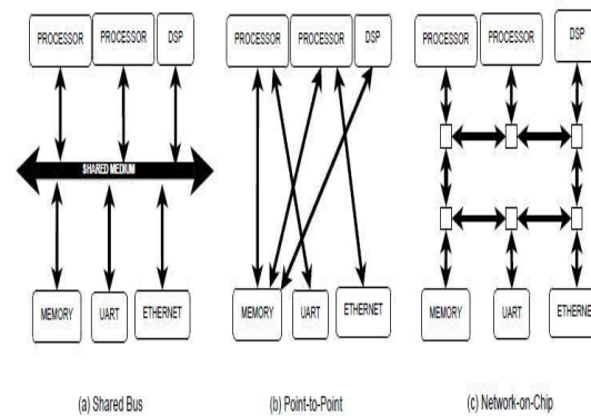
Fig: 1 bus, point to point, NoC communication
