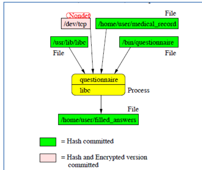
Figure 3-Encryption Model
