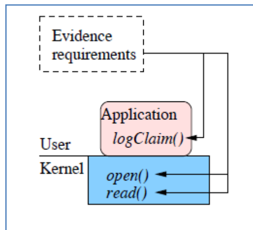
Figure 2-Auditing Model
