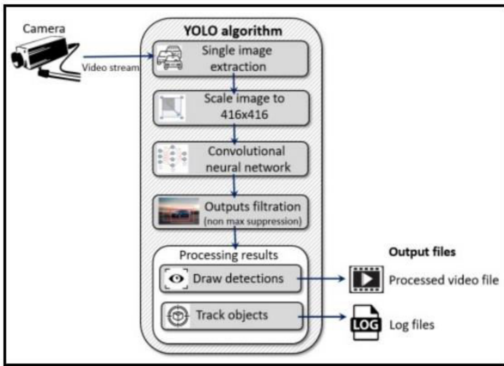
Fig1 : Yolov3 Architecture
