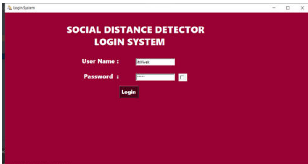
Fig. 6: Login Window
