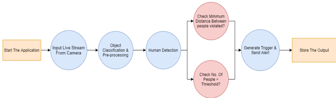
Fig. 4: DFD Level 1
