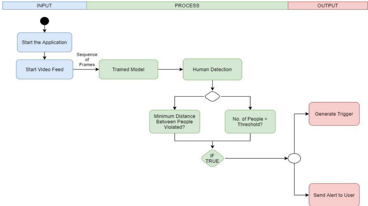
Fig. 1: Activity Diagram
