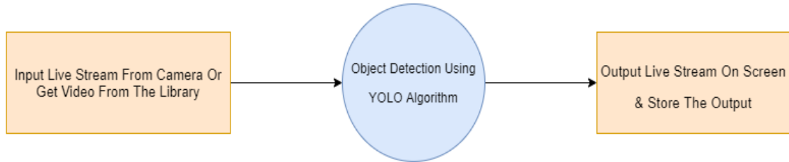
Fig. 3: DFD Level 0
