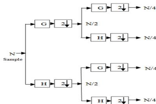
Figure 2: Block Diagram of 2-D DWT
