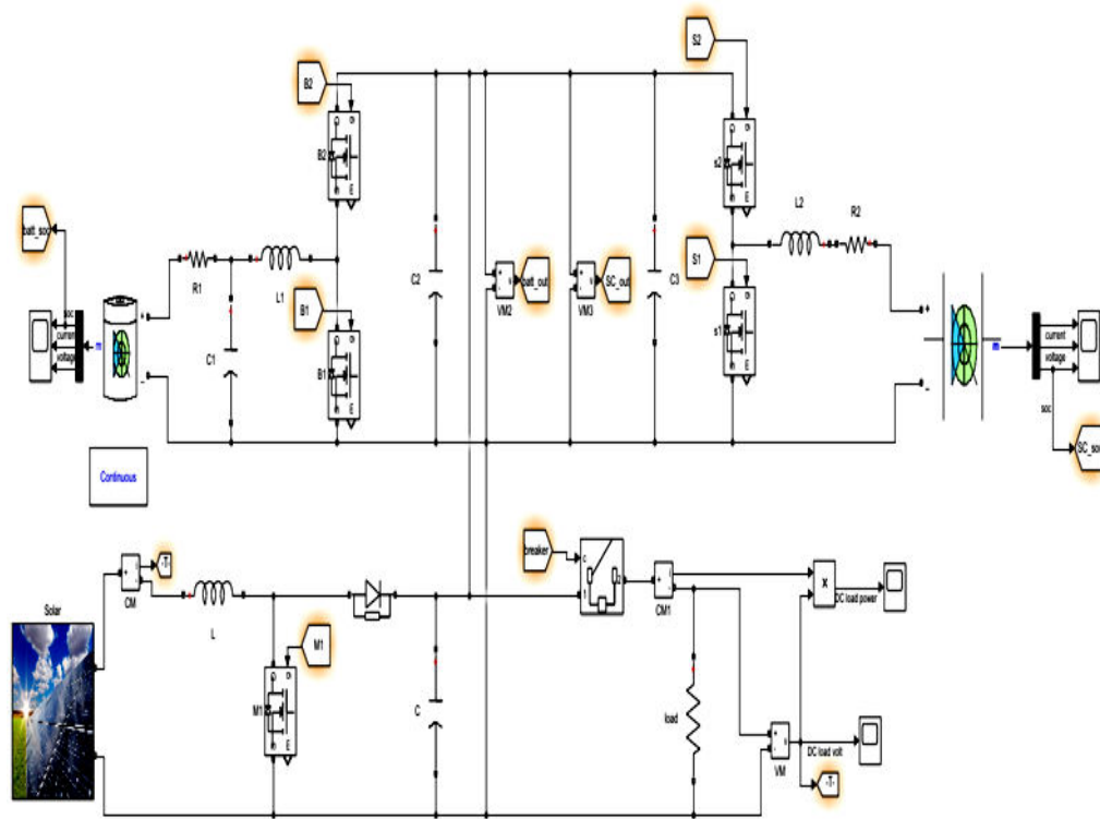
Figure 2: Proposed Model
