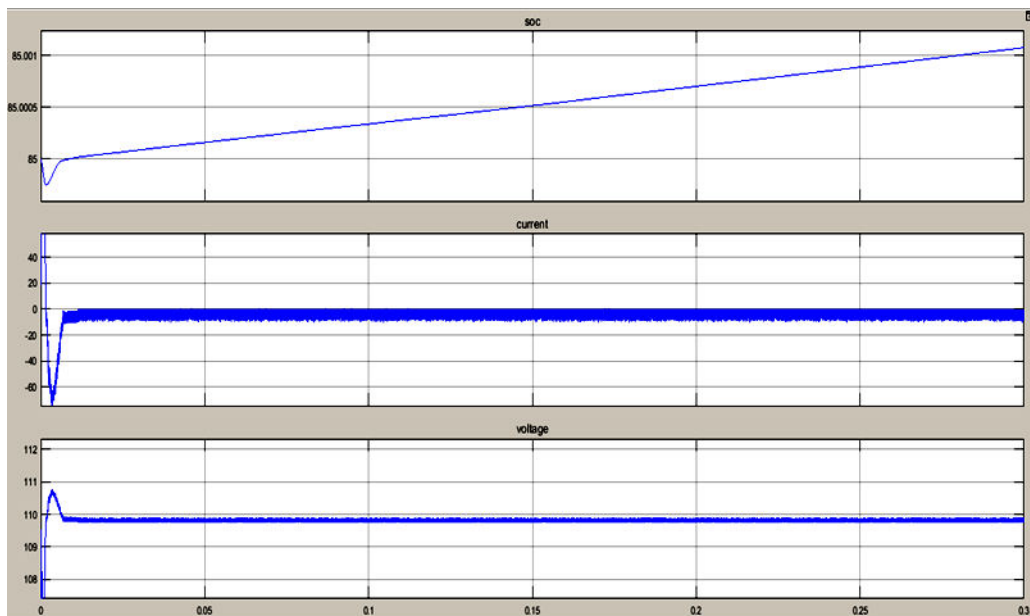
Figure 6: Battery (SOC, Current, Voltage)
