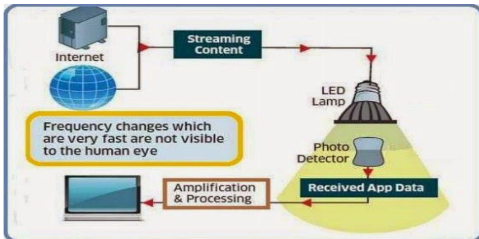
Fig 3: Block diagram of Li-Fi Sub System.
