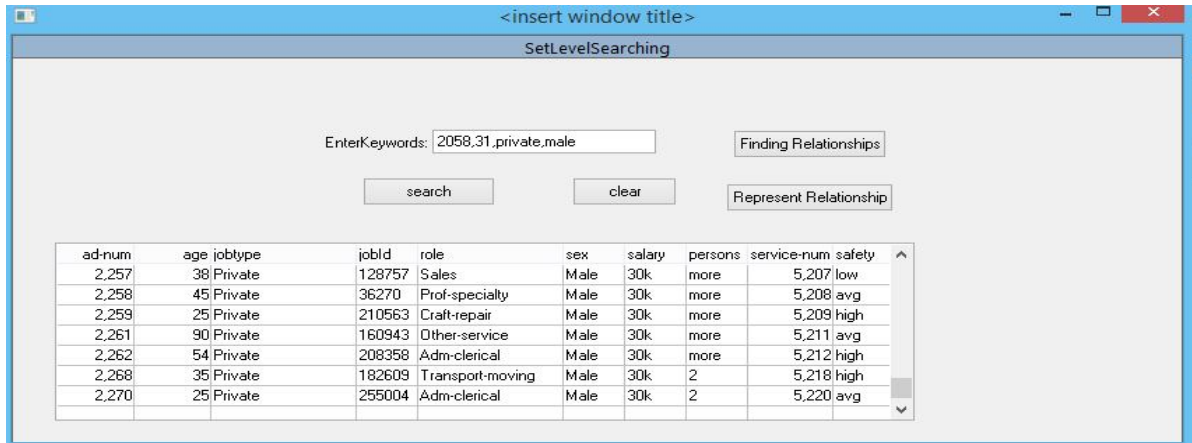
Fig 9: result retrieves when search type is set level searching
