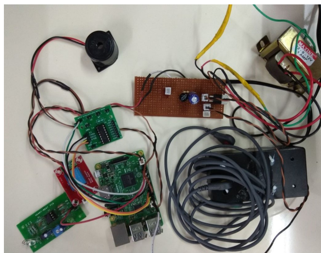
Fig.5 Experimental Setup of the Proposed System
