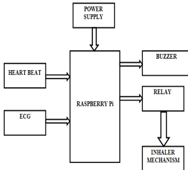
Fig.3 Transmitter Section – Block Diagram
