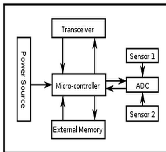
Figure 1.2 The typical architecture of the sensor node
