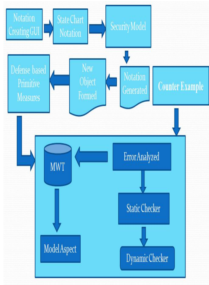
Fig.1. System Architecture Design
