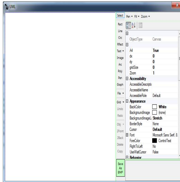
Fig.2. Main Page
