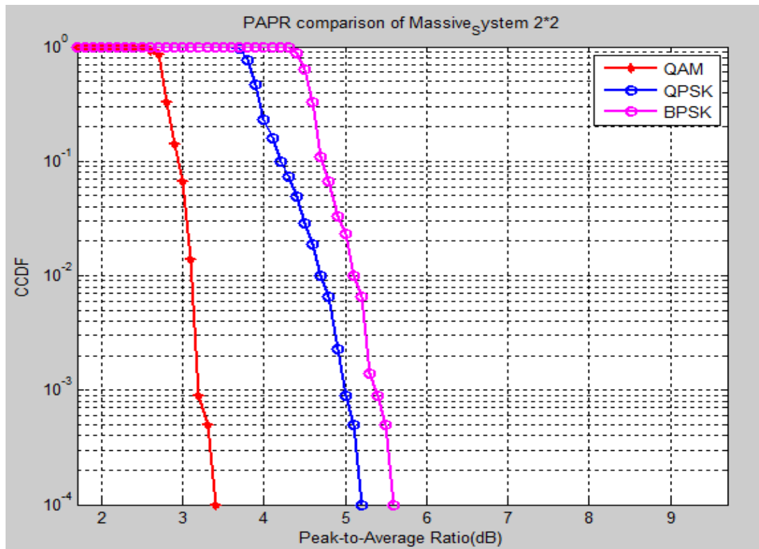
Figure 7: PAPR of Massive 2x2 System with Companding and DCT technique
