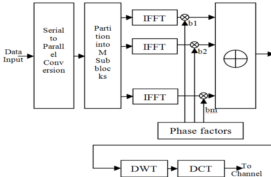
Figure 6: Flow Char of Proposed Methodology
