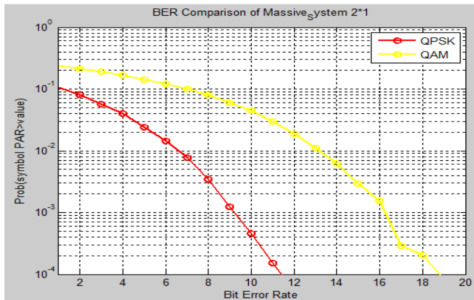
Figure 5: BER Performance of MIMO 2x1 System
