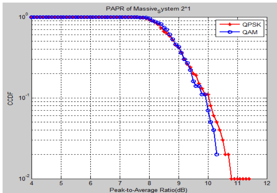
Figure 4: PAPR Performance of MIMO 2x1 System
