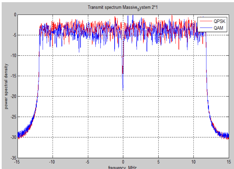
Figure 3: Power Spectral Density of MIMO 2x1 System
