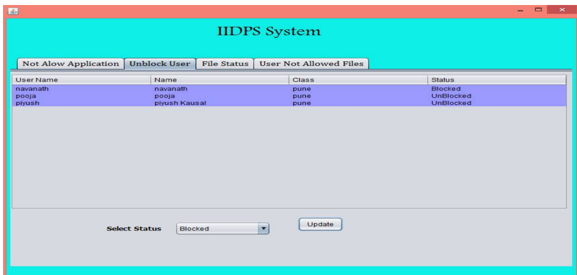
Fig 3: User Status
