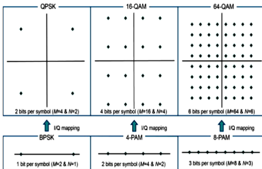
Figure 1: Modulation Schemes
