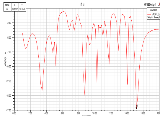
Figure 3: Return Loss Plot in 1GHz – 18 GHz Range
