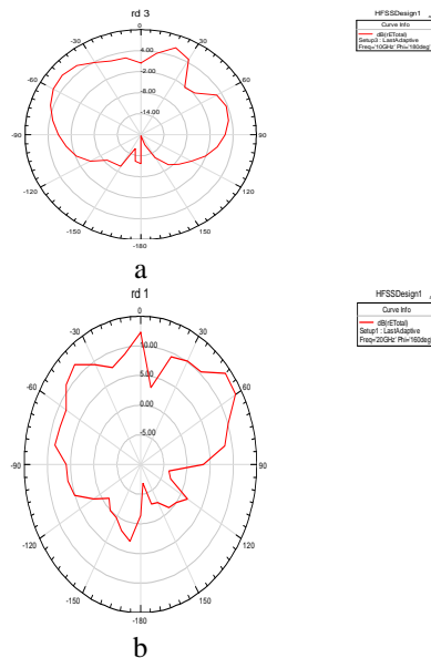
Figure 7: Radiation Pattern
