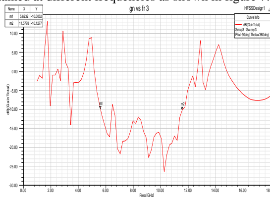
a. 1GHz – 18Ghz Frequency Range
