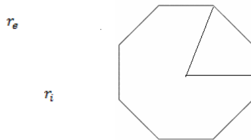
Figure 1: Geometry of Octagonal Sub array
