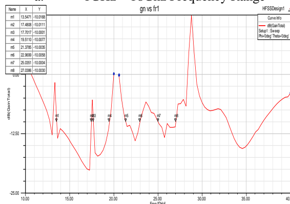
b. 10GHz – 40GHz Frequency Range
