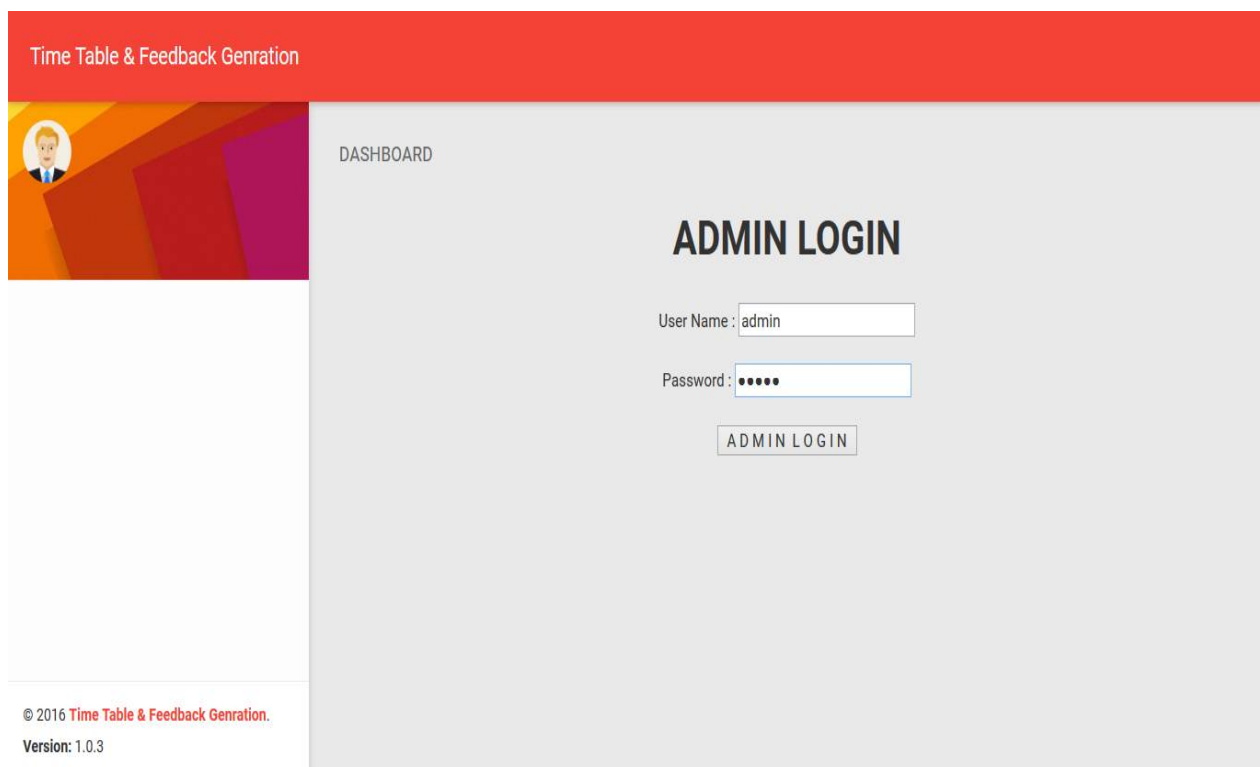
Figure.1 Admin Login
