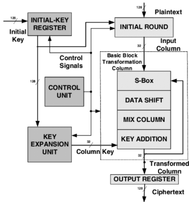
Figure 1: AES block diagram
