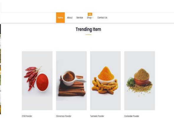
Fig 2. Shop Page
