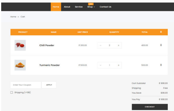
Fig 3. Cart Page
