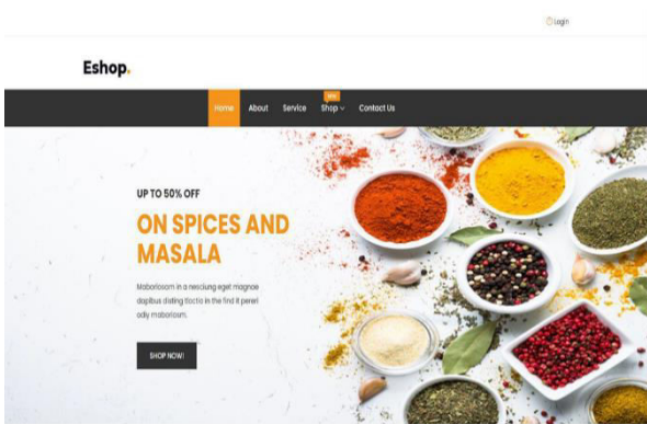
Fig 1. Home Page
