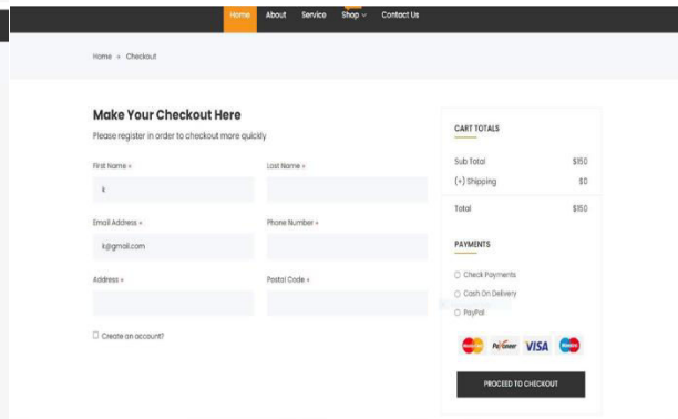
Fig 4. Checkout Page
