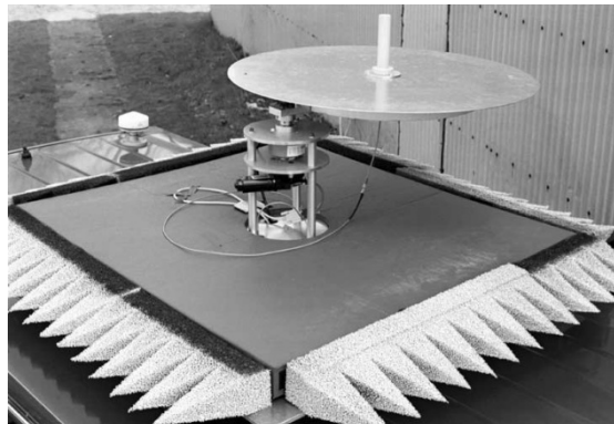
Fig.1: Photograph of the rotating antenna on the vehicle-roof.
