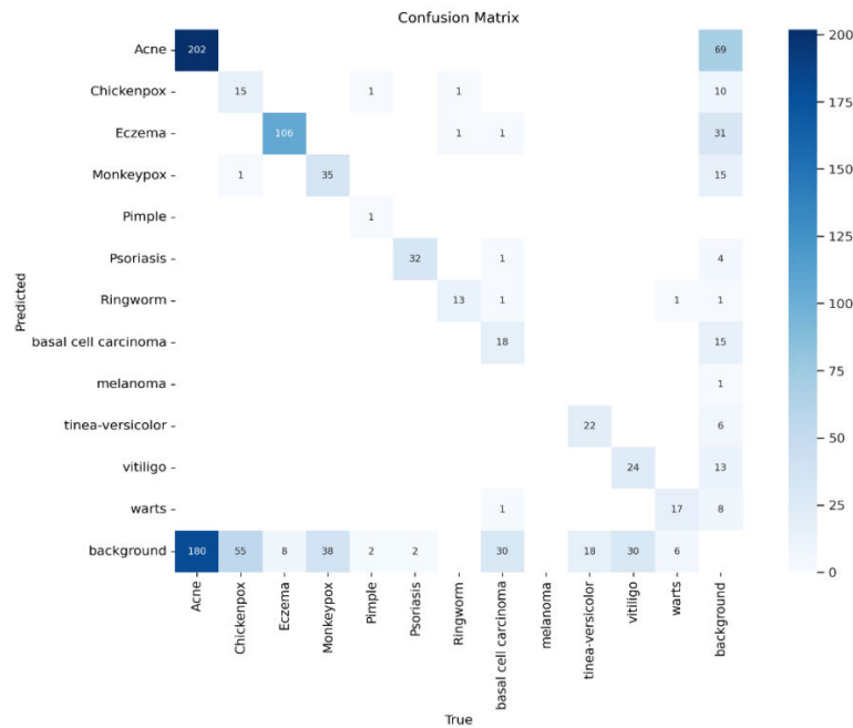
Fig. 4 Confusion matrix of our proposed DermaAITM
