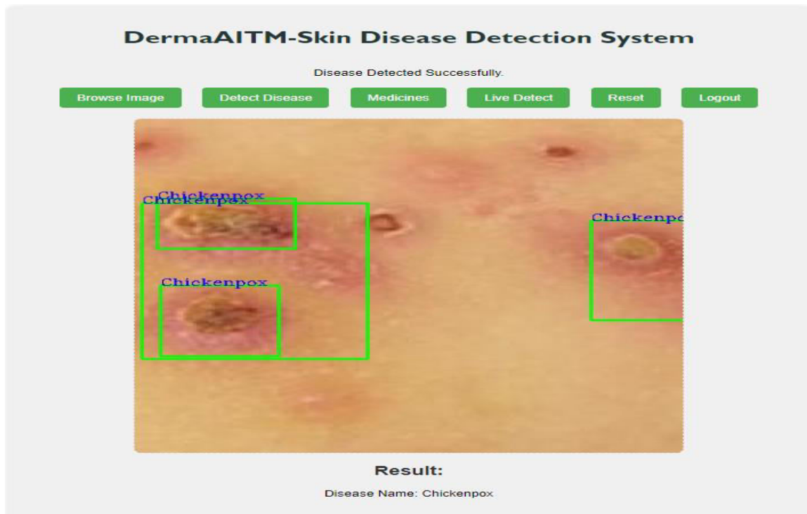
Fig. 6 Identifying the disease name from image
