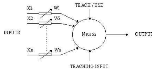
Fig. 5 An MCP neuron
