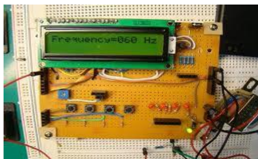
Figure No 5: Frequency counter
