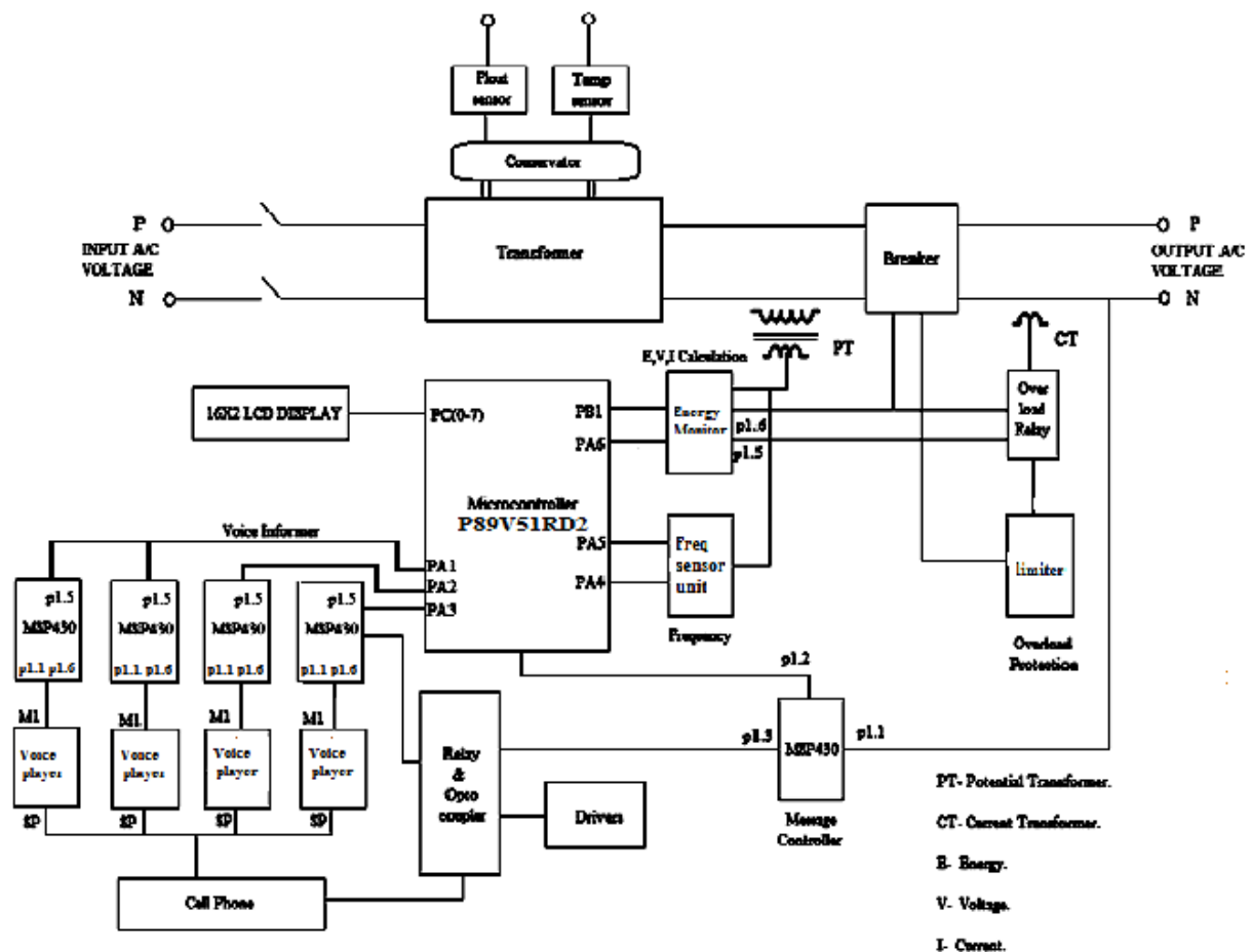
Figure No 1: Block Diagram of Proposed Monitoring System
