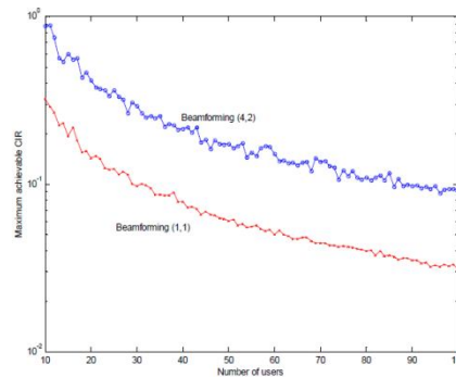
Figure 3. Power Control in MIMO-OFDM
