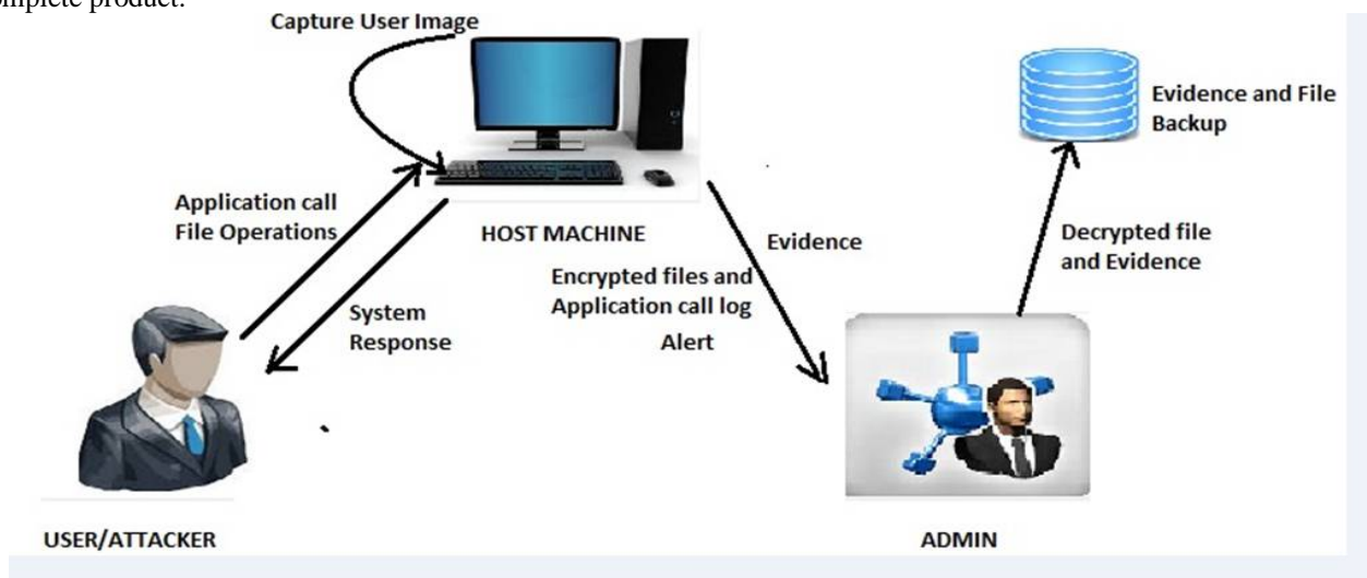
Figure 1: System architecture
