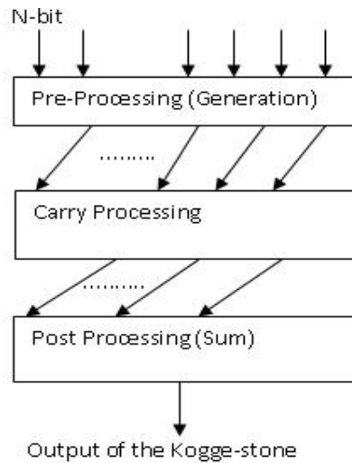
Figure 3: A Block Structure of Kogge Stone Adder bit binary addition
