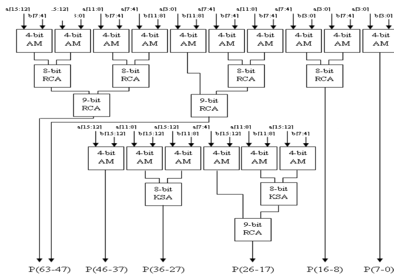
Figure 6: Linear Convolution based on array multiplier and RCA adder
