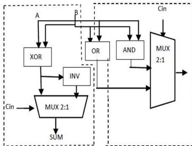
Figure 5: Block Diagram of CBL
