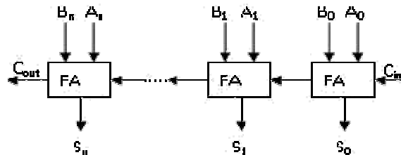
Figure 2: An n-bit Ripple Carry Adder bit binary addition
