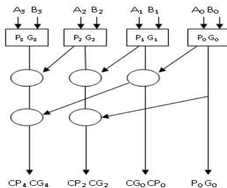
Figure 4: A Functional Diagram of Kogge Stone Adder Stone Adder bit binary addition
