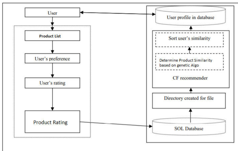
Fig 1. Architecture Diagram
