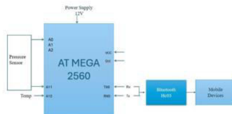
FIGURE 1 BLOCK DIAGARM.
