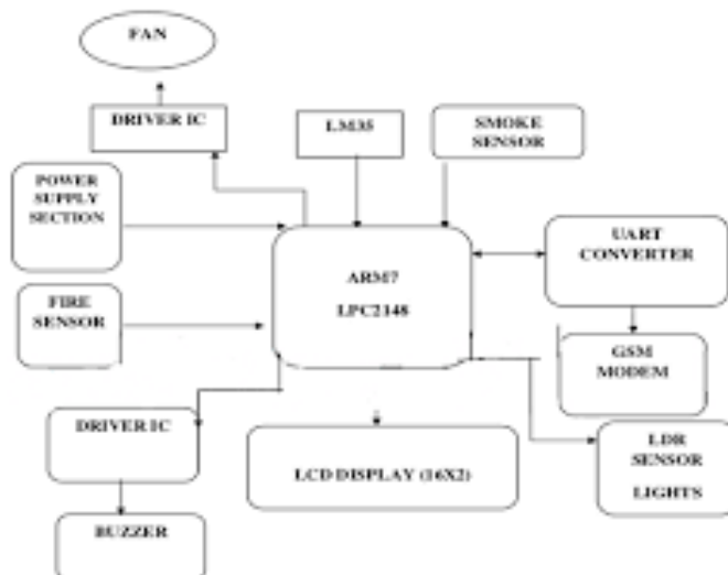
Figure 2. Block diagram of module in ATM using ARM
