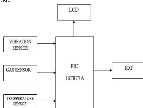
Figure 3. Block diagram of module inside the ATM
