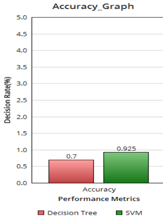
Fig.1 Performance Evaluation
