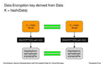
Fig 4. Convergent Encryption
