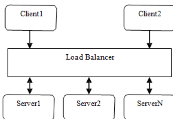
Figure 1. Load balancer
