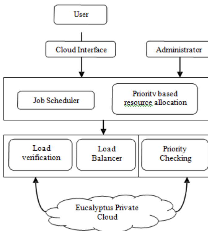
Figure 2. Cloud Architecture
