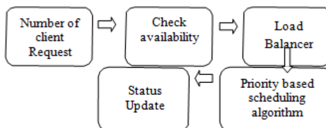
Figure 3. Load balancing workflow
