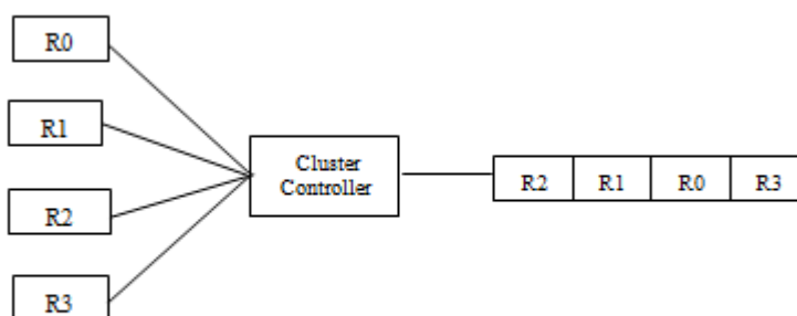
Figure 4. Priority based scheduling
