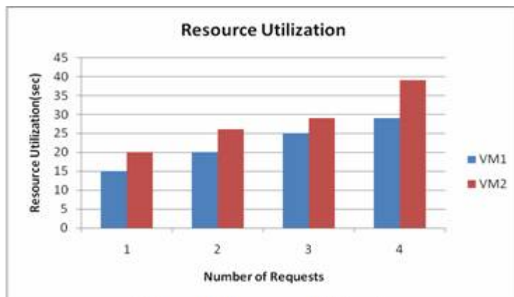
Figure. 9. Resource Utilization
