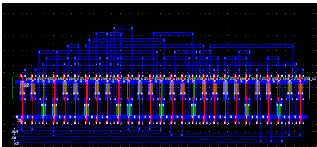
Figure 5: Layout of 18-TSPCFF
