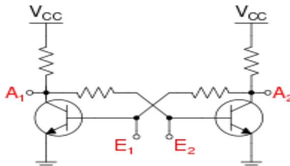
Figure 1: A traditional (simple) flip-flop circuit
