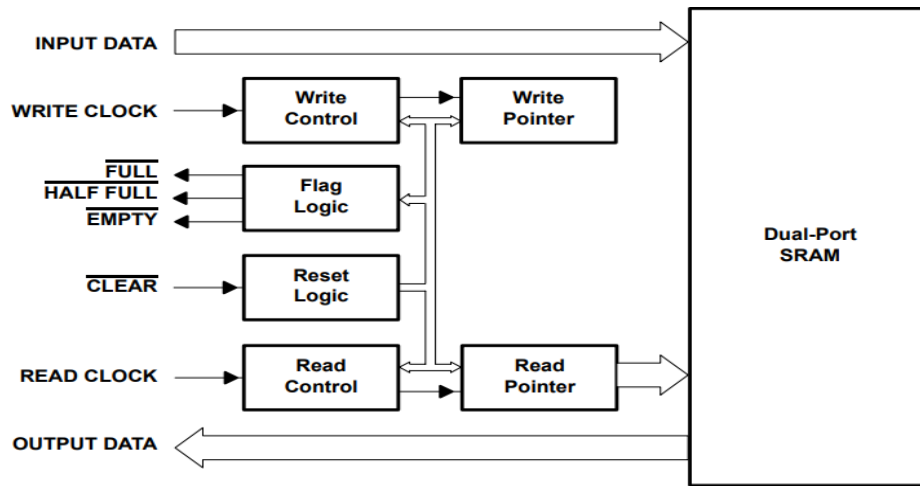
Figure 2: Block diagram of FIFO with storage
