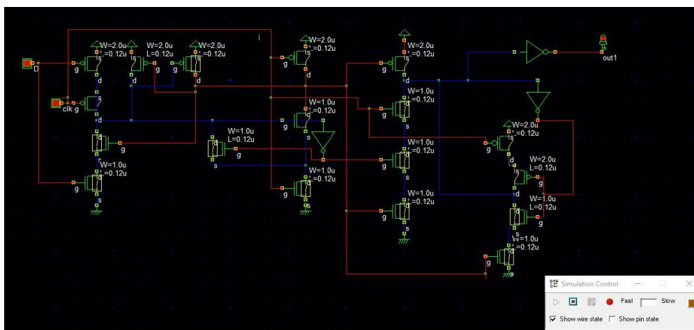
Figure 4: Proposed 18-transistor single-phase clocked (TSPCFF)
