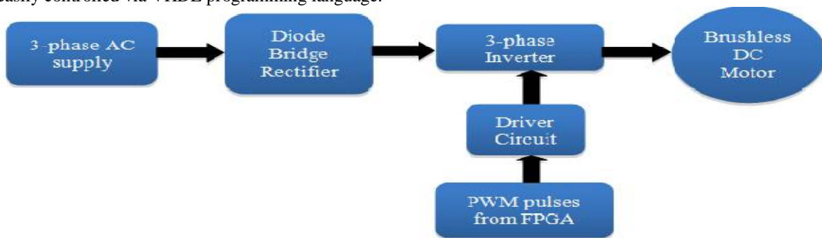
Fig 2: Block diagram
