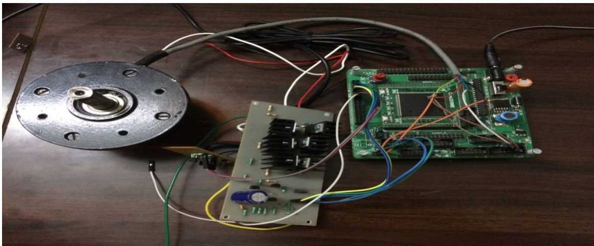
Fig 4: Proposed hardware
