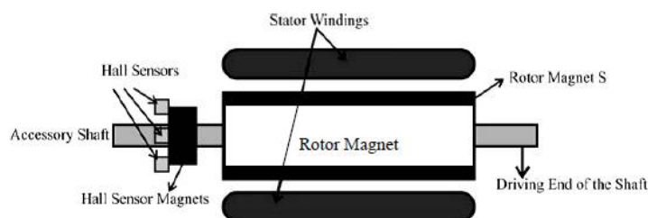
Fig. 1: BLDC Motor with Hall Sensors
