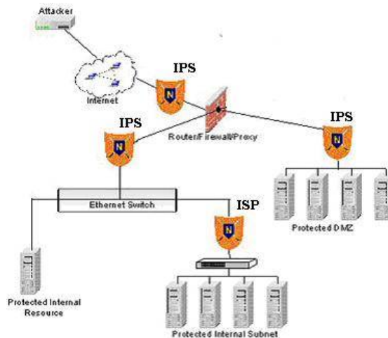
Fig. 10. Network based intrusion prevention system [64].
