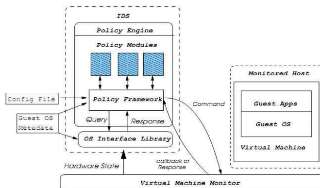
Fig. 9. VMI-basedIDS architecture [26].
