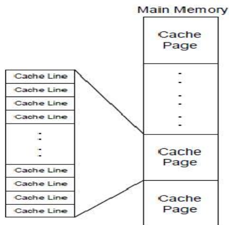
Fig. 2: Cache Page [8]
