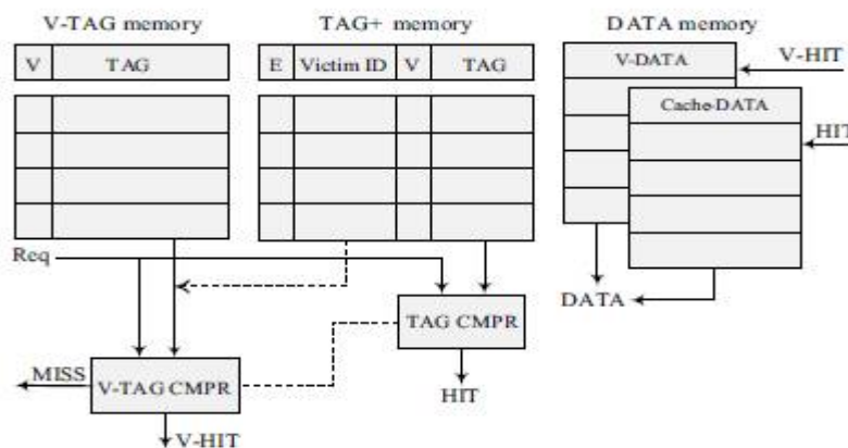
Fig 7: Cache Structure [1]
