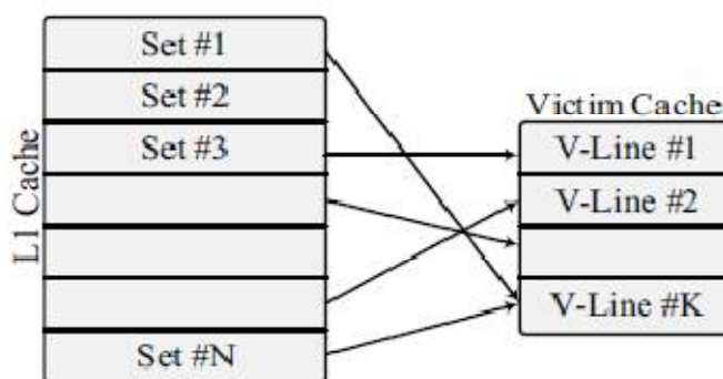
Fig 8: Cache mapping structure [1]
