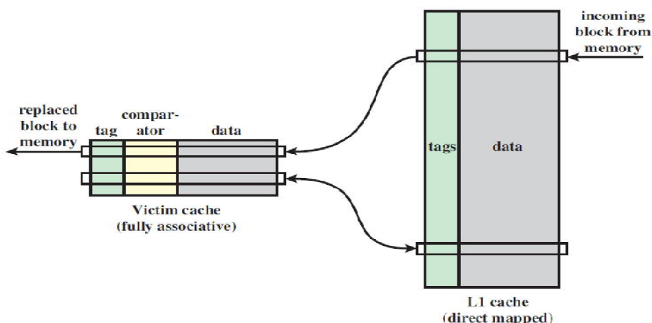
Fig. 6: Victim Cache Operation[5]
