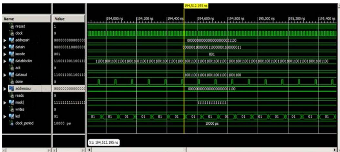
Fig 10: Victim Cache simulation
