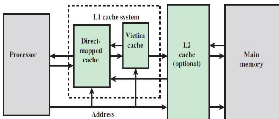
Fig 5: Memory hierarchy for the victim caching scheme.[5]
