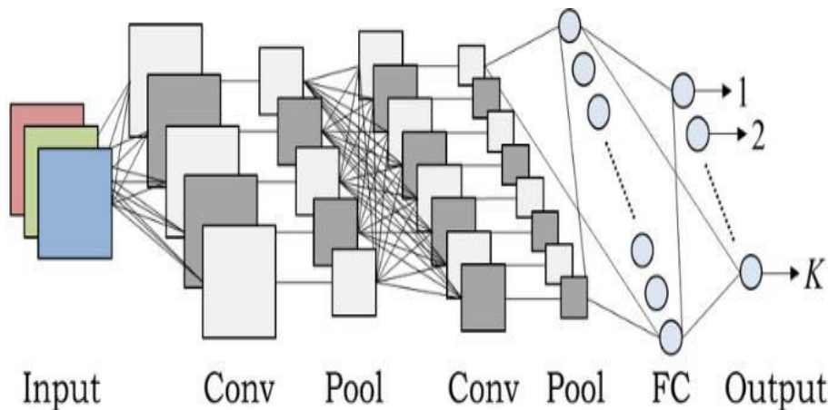
Fig 2 CNN architecture
