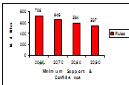
Figure 2. Number of Rules generated for fixed minimum support varies in confidence
