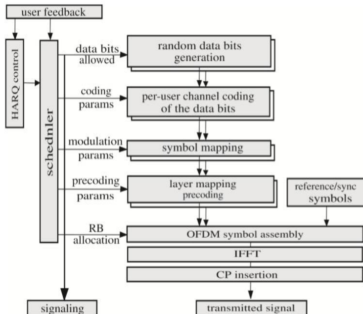
Figure 4: LTE downlink transmitter structure
