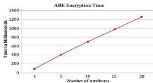
Fig 3. Encryption time of ABE
