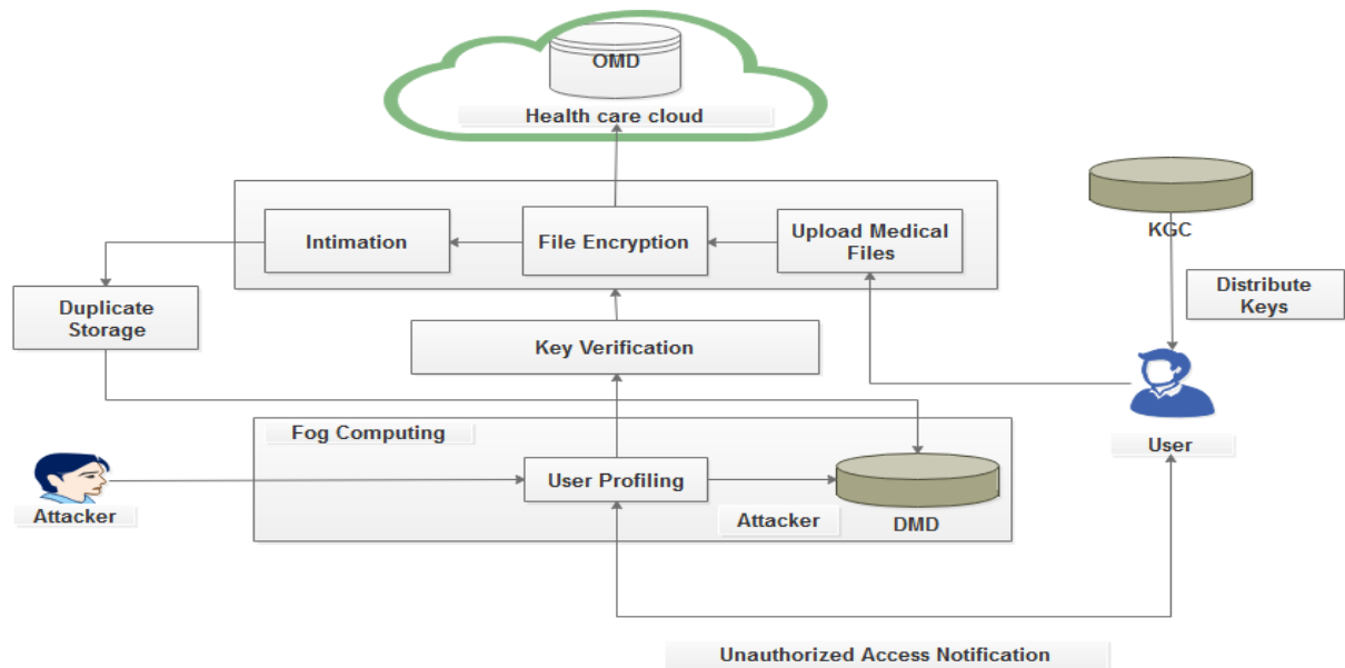
Fig 1. Architecture diagram
