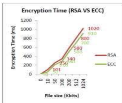
Fig 2. Encryption time of RSA and ECC
