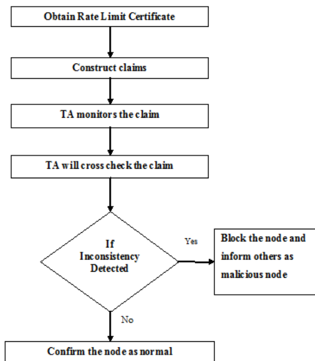
Fig. 1 System Design of Count Restricting Approach
