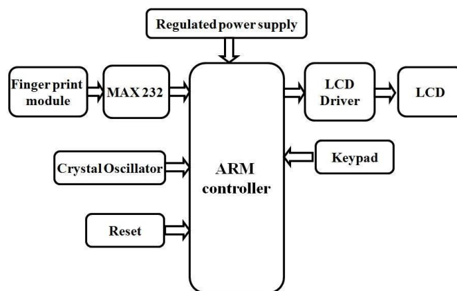
Fig. 1. Block diagram of biometric voting system
