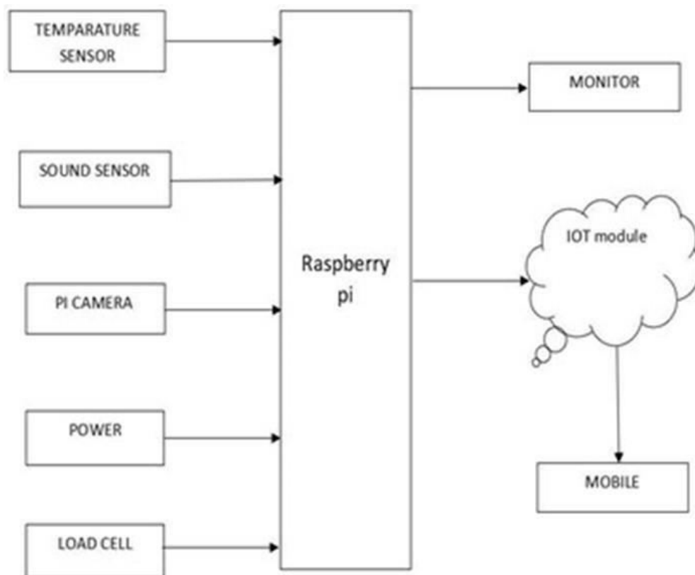
Fig.Block Diagram
