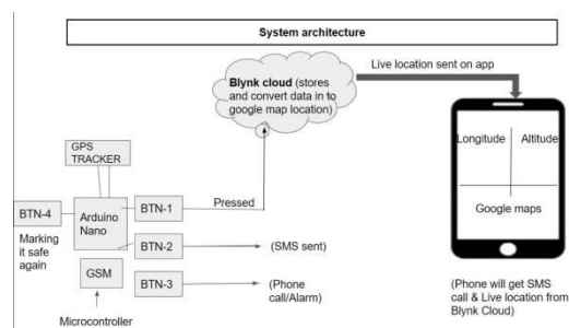
Fig: System Architecture for safety notification
