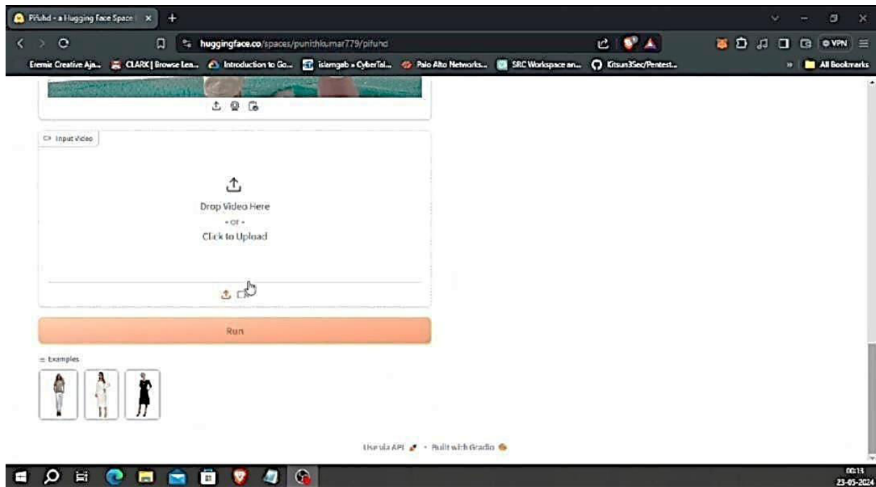
Fig 1 – User Interface
