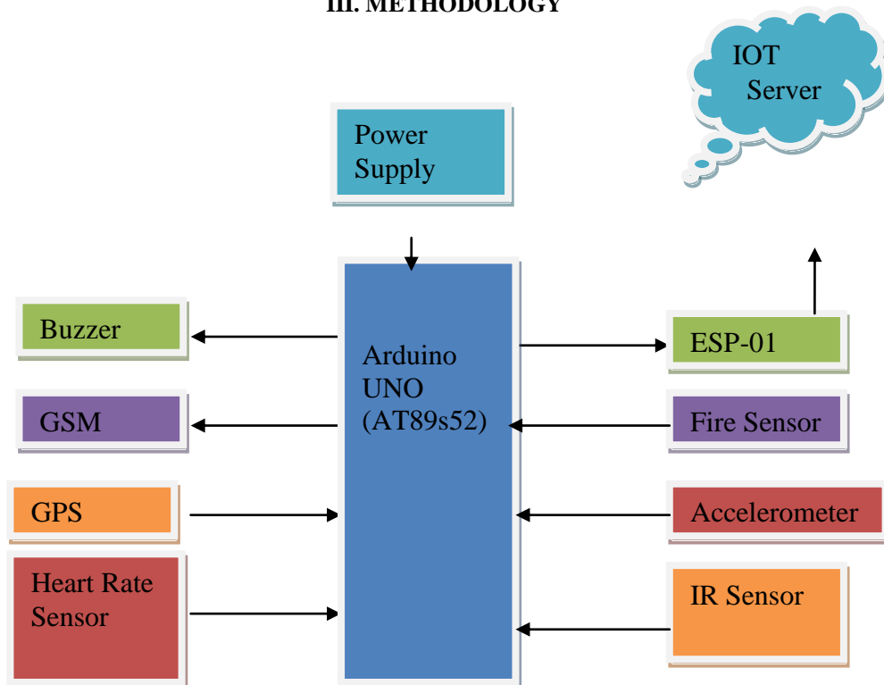
Fig. 1: Vehicle Monitoring and Accident Alert System
