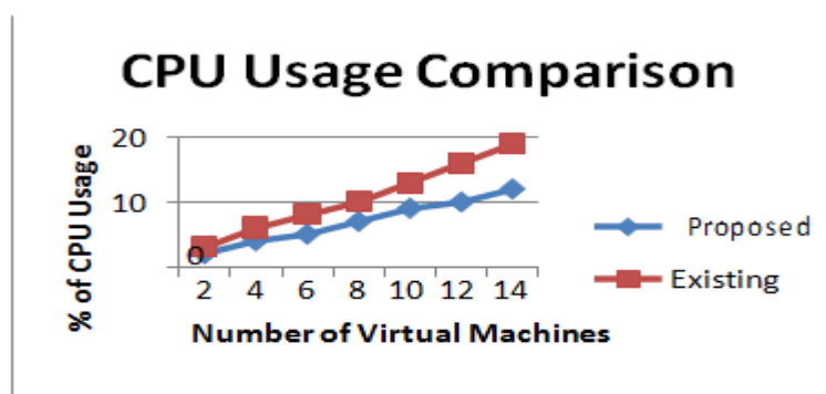
Fig. 6. Performance comparison in terms of CPU cycles
