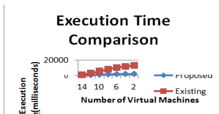
Fig. 5. Performance comparison in terms of execution time
