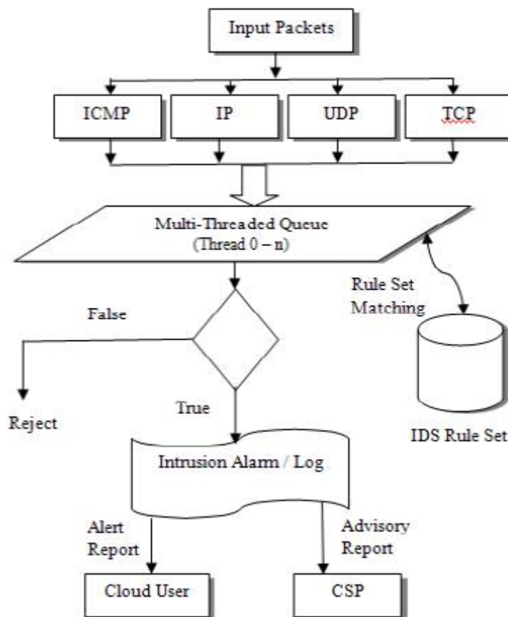
Figure 3. Flow Chart of Multi-Threaded Green cloud IDS Model [6]
