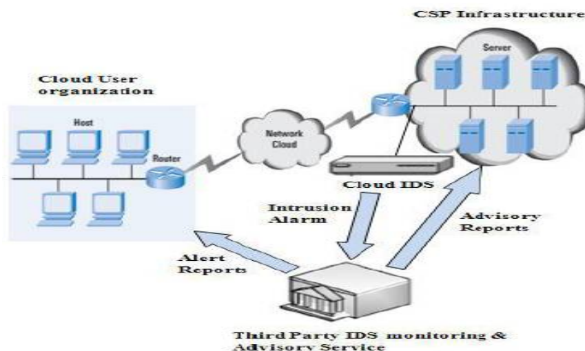
Figure 2. Proposed Green cloud IDS Model [6]
