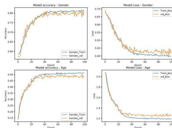
Fig. 7. Accuracy vs Epoch and Loss vs Epoch
