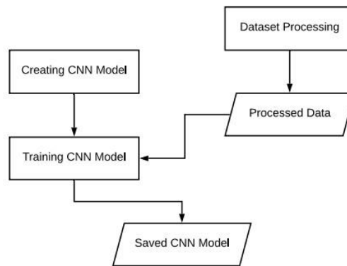
Fig. 1. Training Phase
