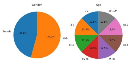
Fig. 3. Dataset Distribution
